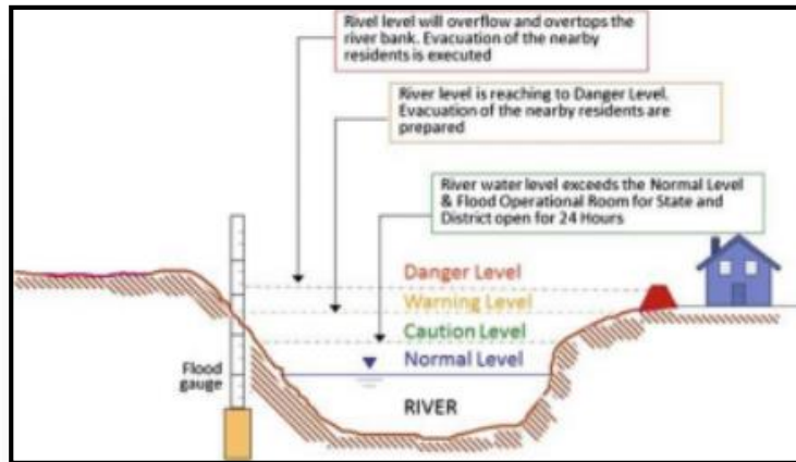
Fig 3. The standard of critical river levels termed by DID Malaysia (Department of Drainage and Irrigation Kelantan, 2014)
